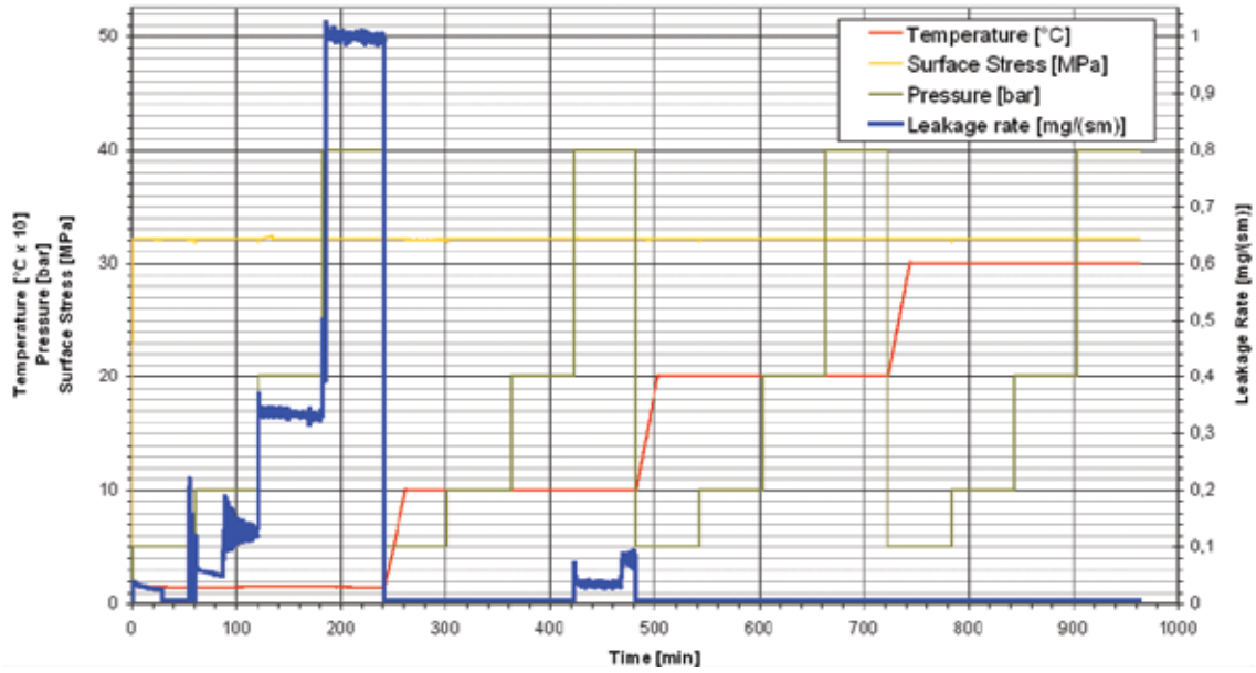
High Temperature Leakage Test with N 2 Doniflex GR-A, 2 mm
